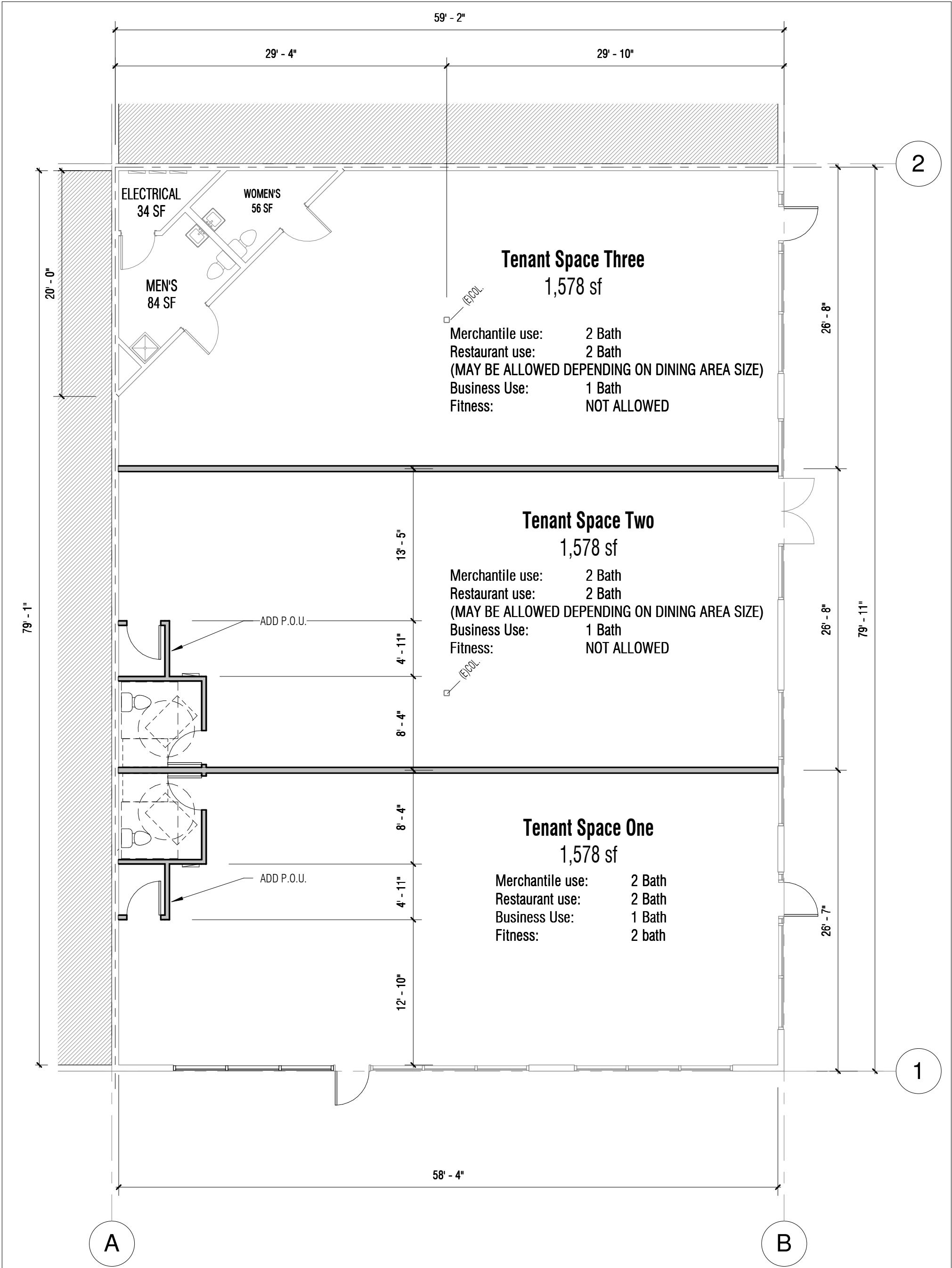
1 FLOOR PLAN 1/8" = 1'-0"
